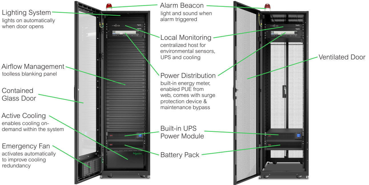
Contained enclosure for commercial applications and semi-controlled environments.
